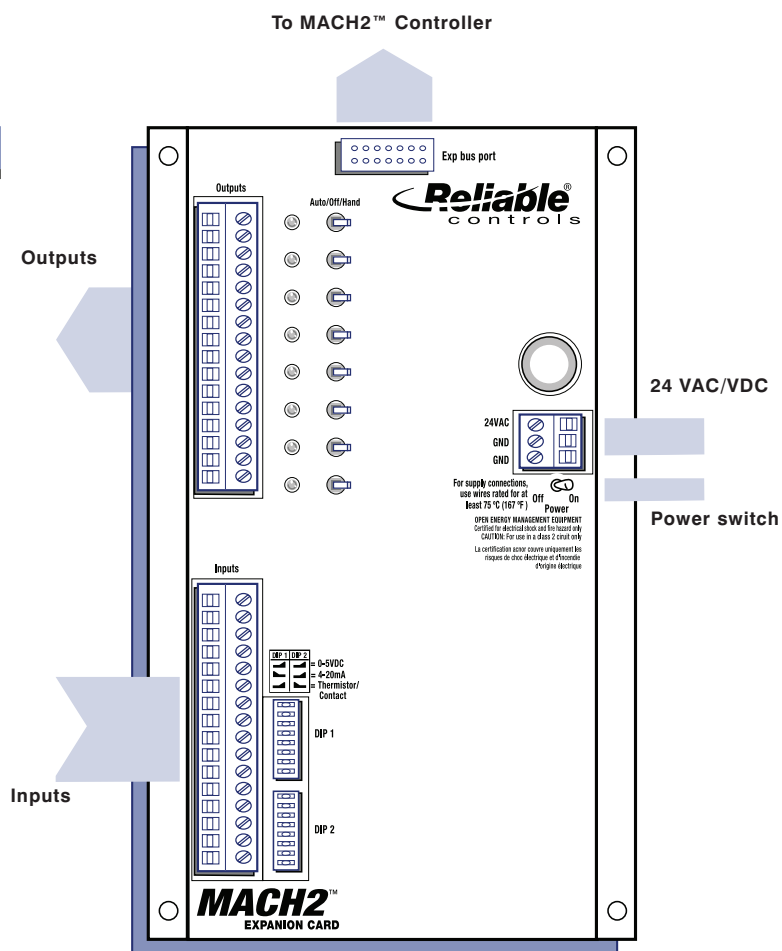
MACH2 ™ Expansion Card
